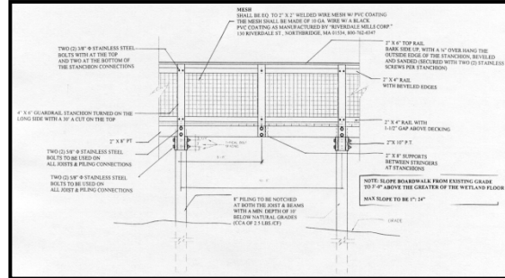
PROPOSED ELEVATION
