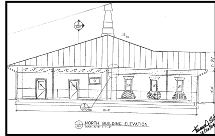
Proposed
